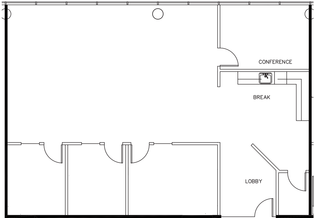
KEY PLAN
